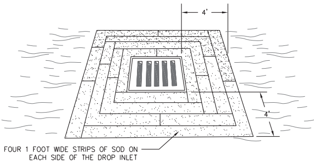
Figure 4. Sod Inlet Protection Installation Requirements (Sd2-S)
