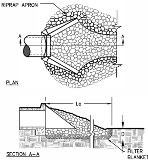
Figure 1. Outlet Protection for a Well-Defined Channel
