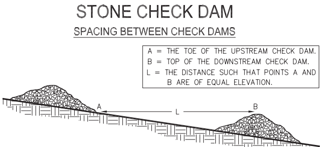
Figure 1. Stone Check Dam Spacing Requirements
