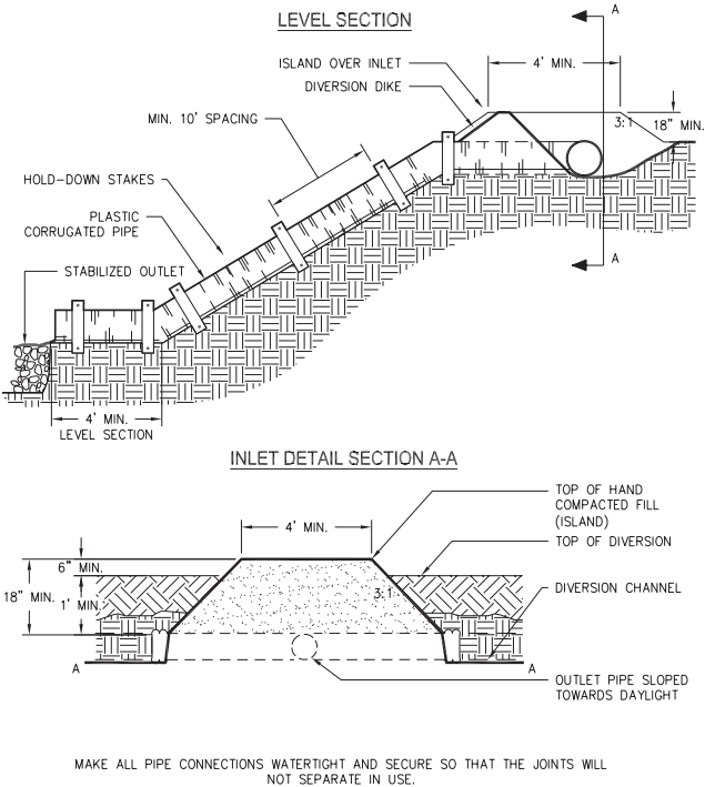
Figure 1. Temporary Downdrain and Inlet Detail
