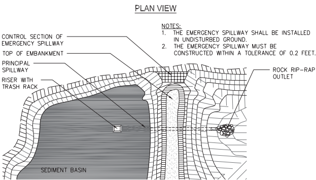
Figure 1. Components of a Typical Temporary Sediment Basin
