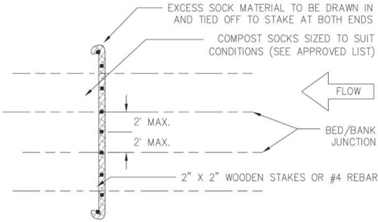
Figure 1. Compost Filter Sock Installation Requirements
