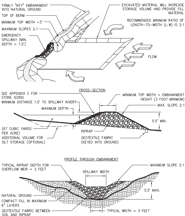
Figure 3. Rock Outlet
