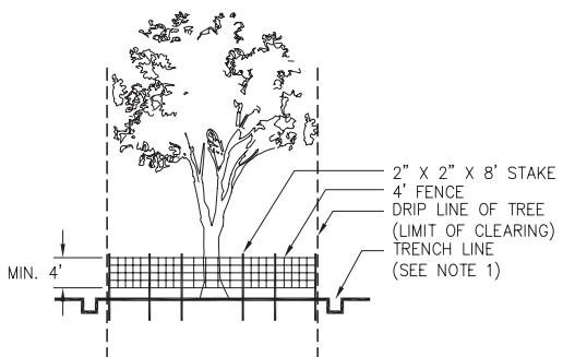
Figure 2. "Snow" Fence Installation
