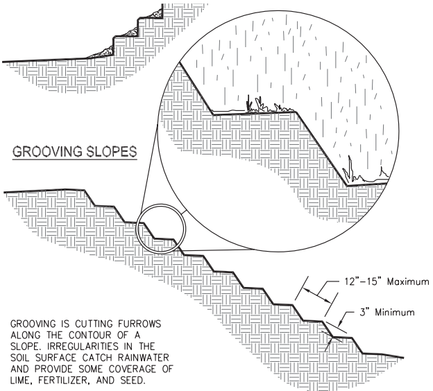
Figure 2. Grooving Slopes
